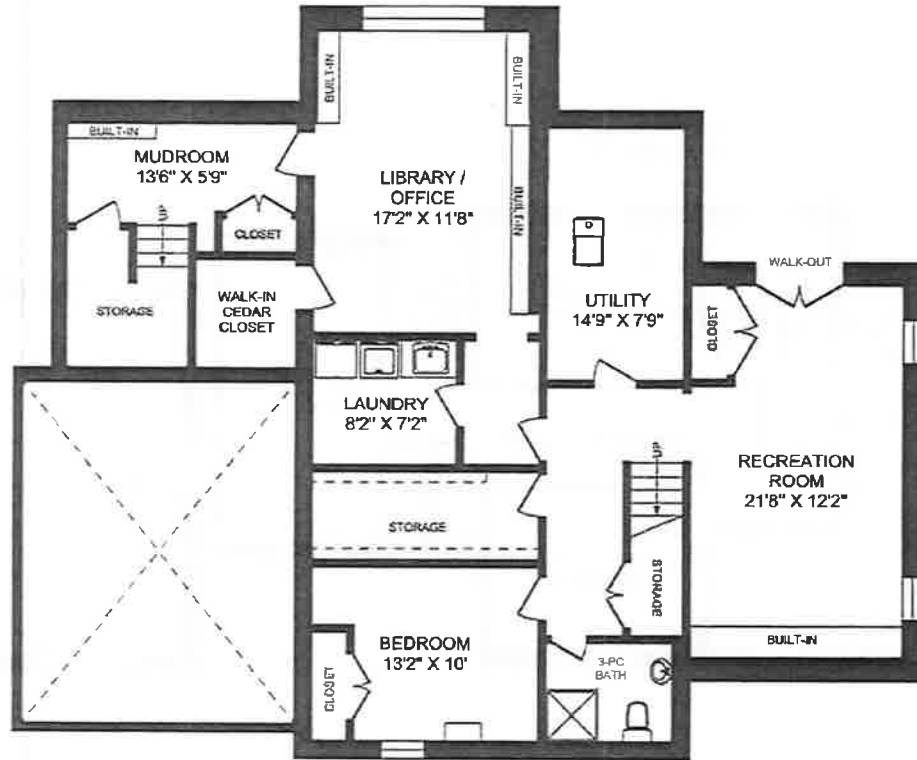
LOWER LEVEL 1492 SQUARE FEET
